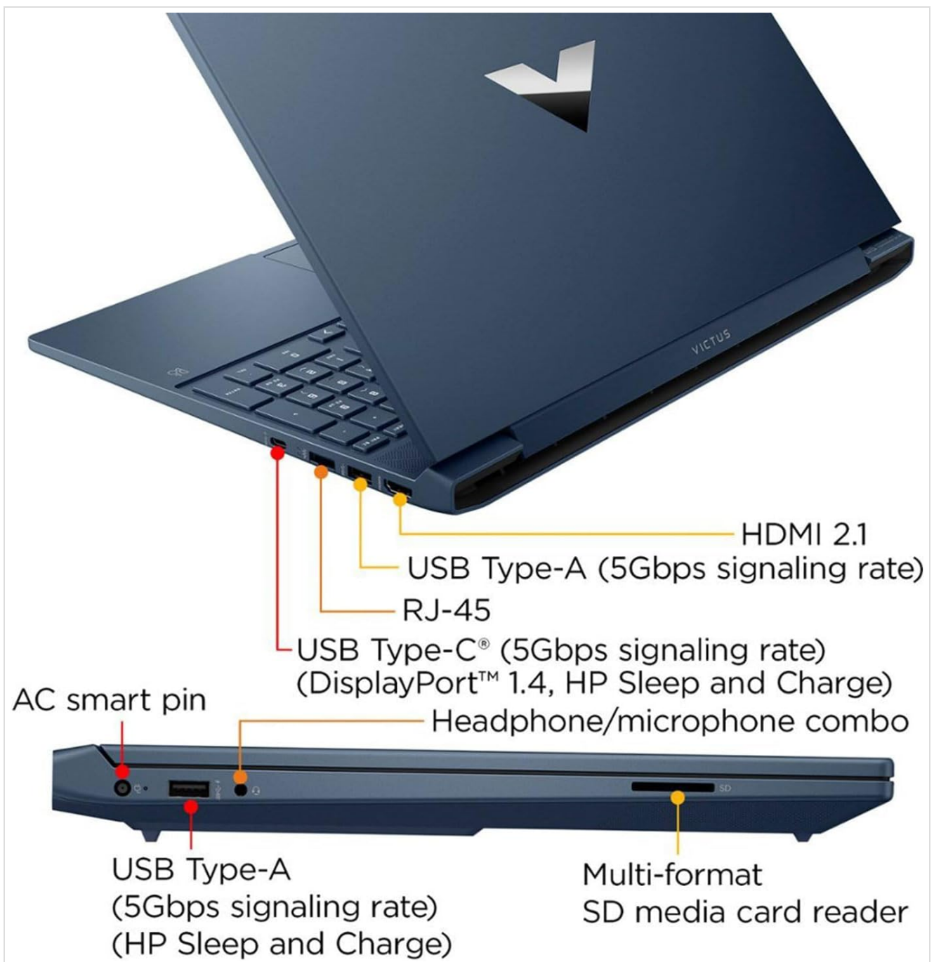
Image: Diagram illustrating the various ports available on the HP Victus laptop, including USB, HDMI, and the SD card reader.
