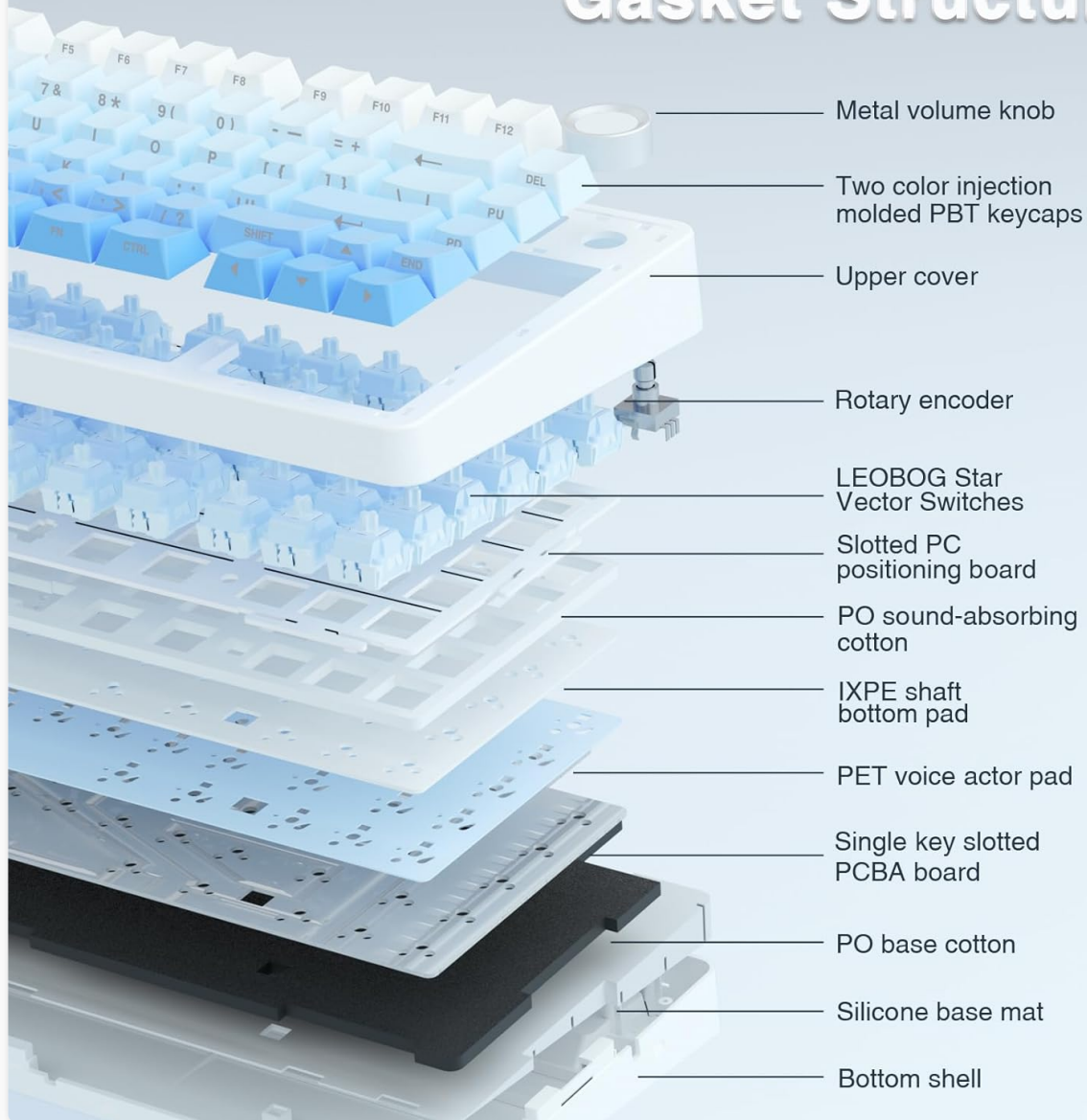
Diagram illustrating the hot-swappable PCB sockets and LEOBOG Star Vector switches, showing how they can be easily replaced.
