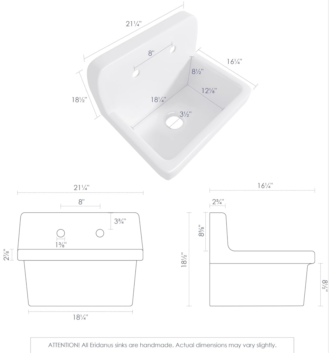
Image 8.1: Detailed dimensions of the Eridanus utility sink.
