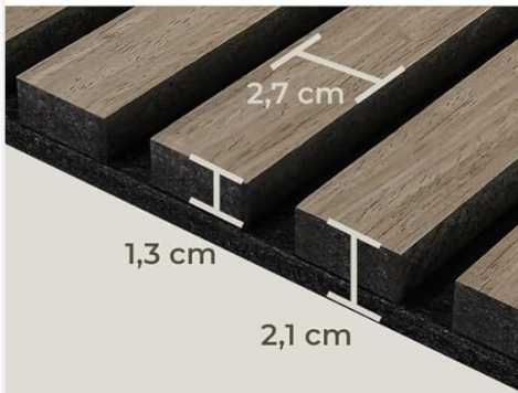
Image: Technical drawing with precise dimensions of the acoustic panel.
