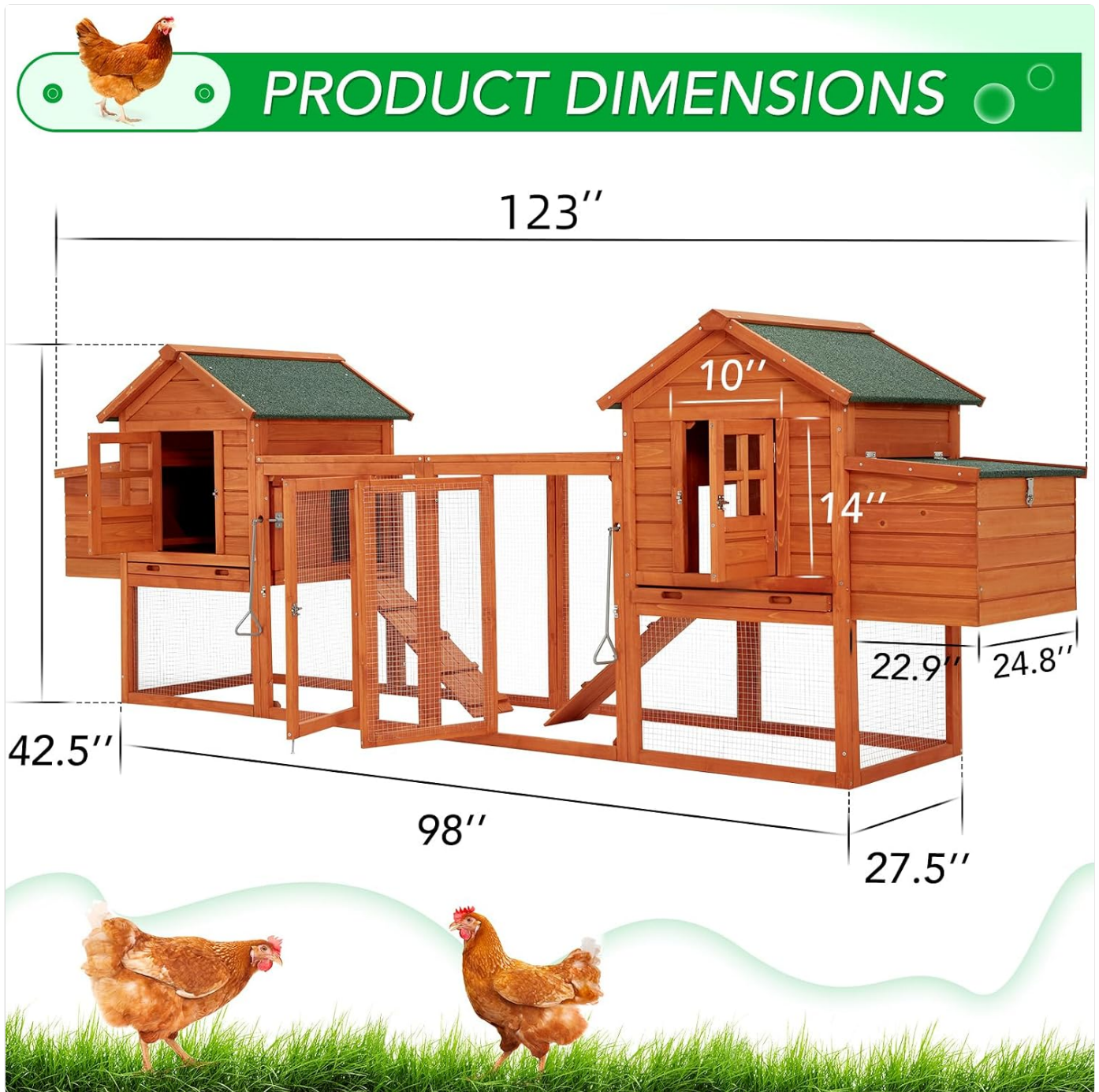
Figure 4.1: Overall dimensions of the chicken coop. The coop measures 123 inches in length, 27.5 inches in width, and 42.5 inches in height. This diagram is crucial for planning the placement of the coop in your yard.
