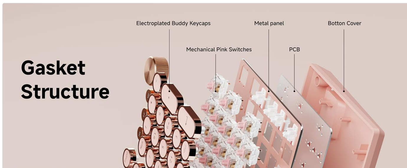
Figure 3: Internal Gasket Structure for improved typing experience.
