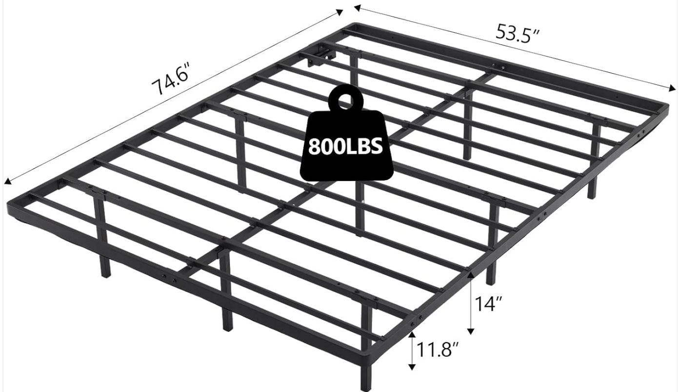
Image 4.2: Visual representation of the bed frame's dimensions (74.6"L x 53.5"W x 14"H) and its robust 800 lbs weight capacity.
