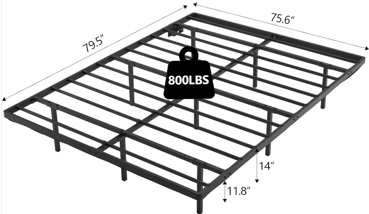
Image 8.1: Key dimensions and weight capacity of the King size bed frame.
