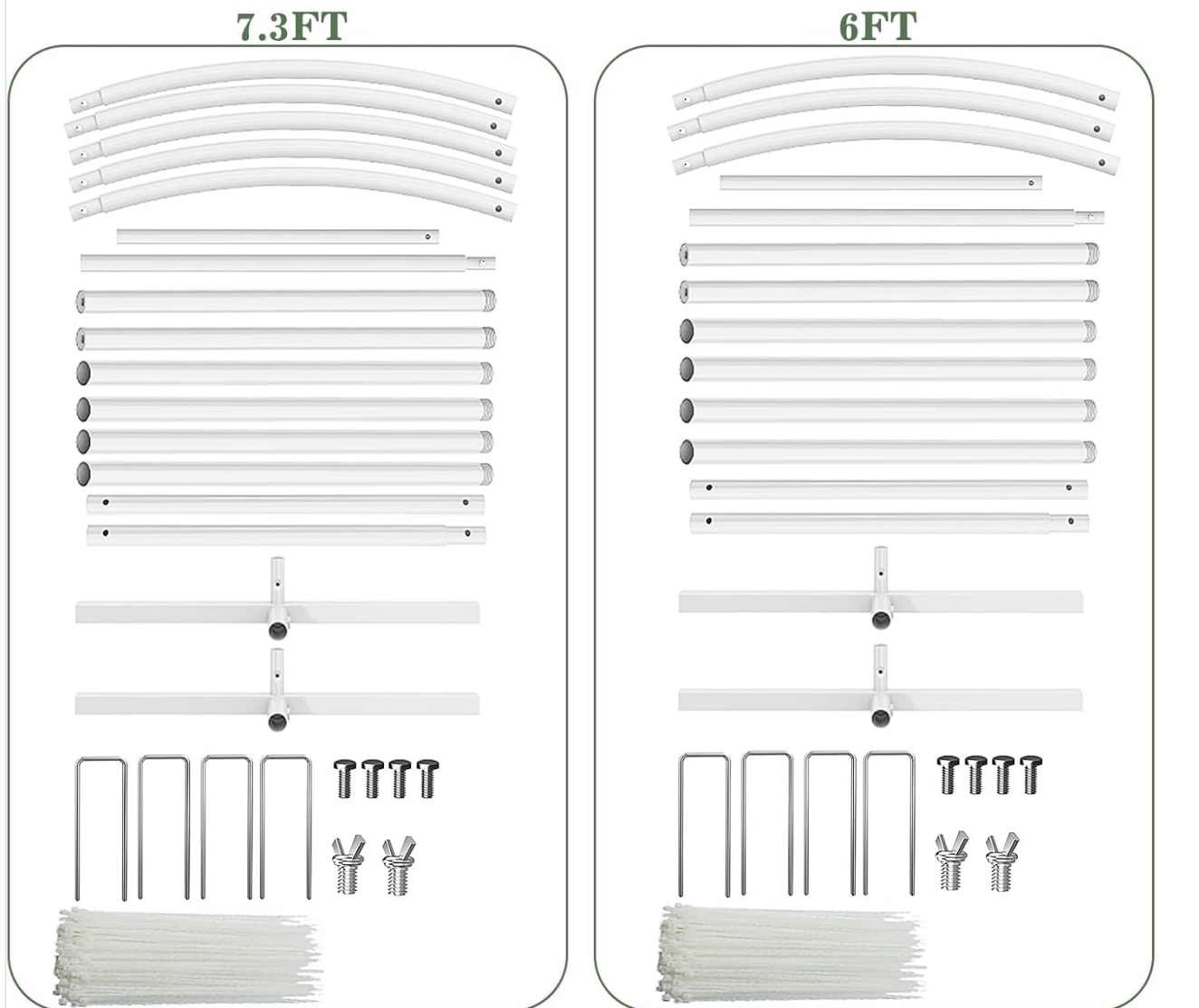
Figure 3.1: Product Accessories List for 7.3FT and 6FT Arches
