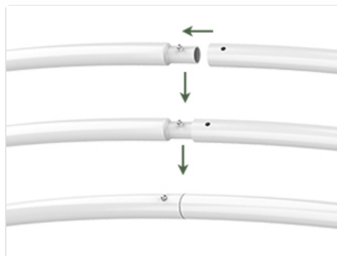
Figure 4.2: Arch Pipe Connection Detail
