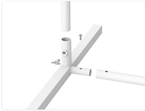
Figure 4.3: Base Connection Detail
