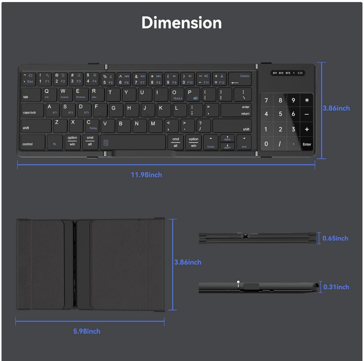
Image: Detailed dimensions of the keyboard in both unfolded and folded states.
