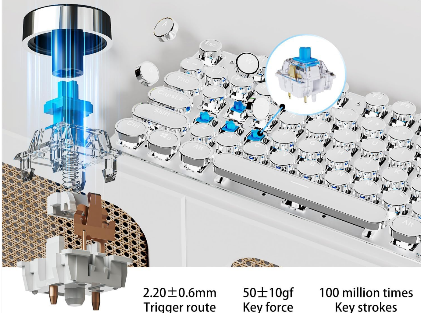
Figure 6: Detailed view of the Mechanical Blue Switch, highlighting its trigger route, key force, and key strokes durability.
