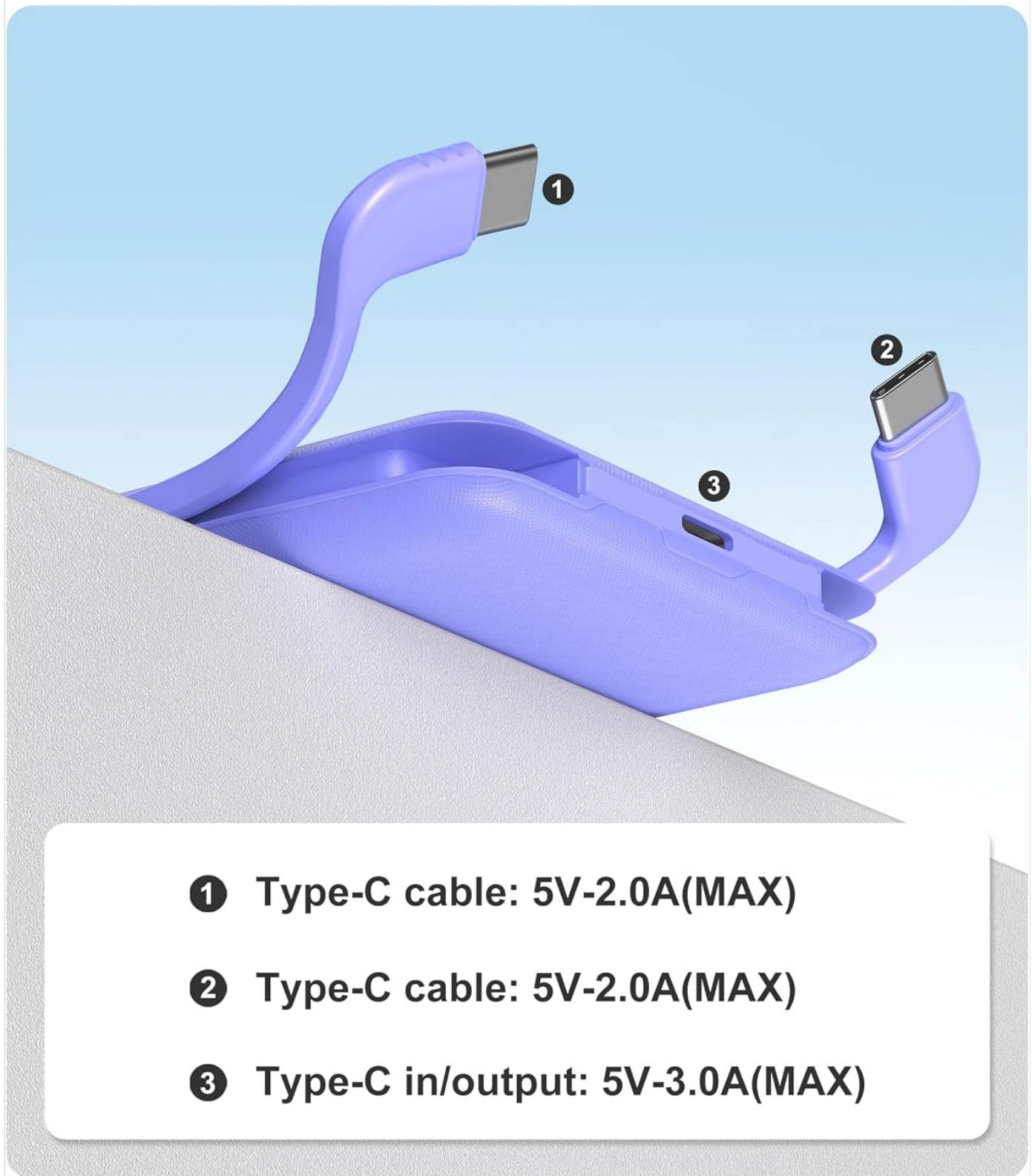
Figure 3: Built-in Cables and Output Ports
