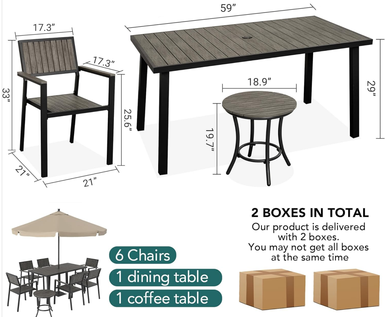
Image 2.1: Overview of included components and their approximate dimensions.
