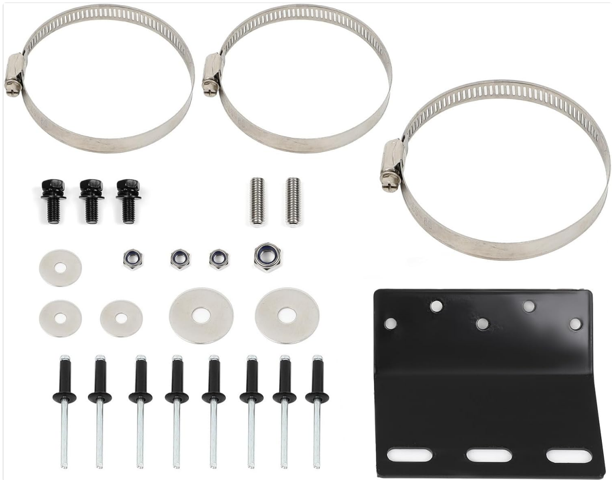
Image 2: Close-up view of the various bolts, nuts, washers, clamps, and mounting plate included in the hardware kit.
