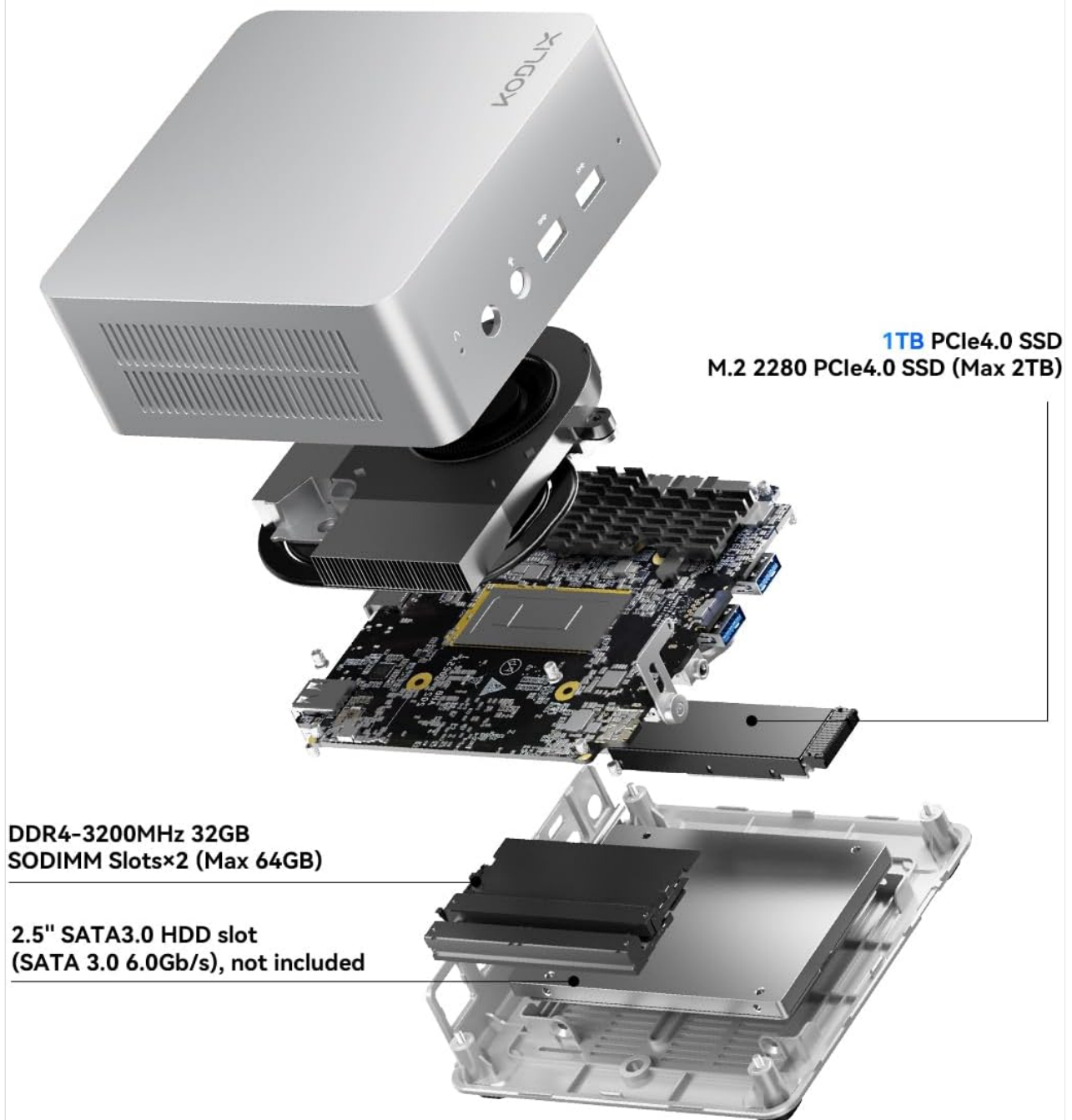
Figure 2.1: Internal view of the KODLIX GD90 Mini PC, highlighting the SSD and RAM slots for expansion.
