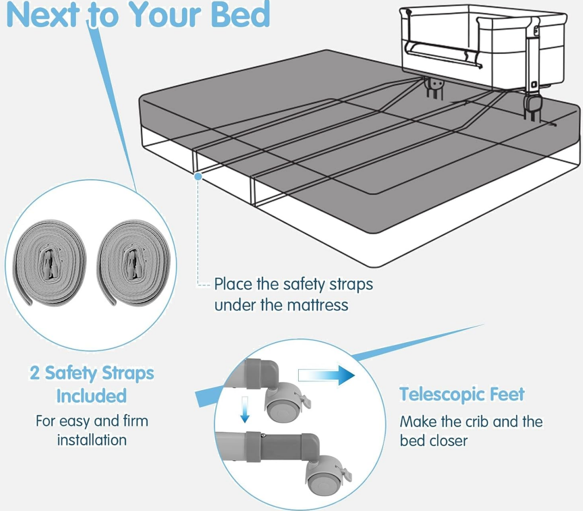
Image: Diagram showing how to securely install the bassinet next to an adult bed using the safety straps and telescopic feet.
