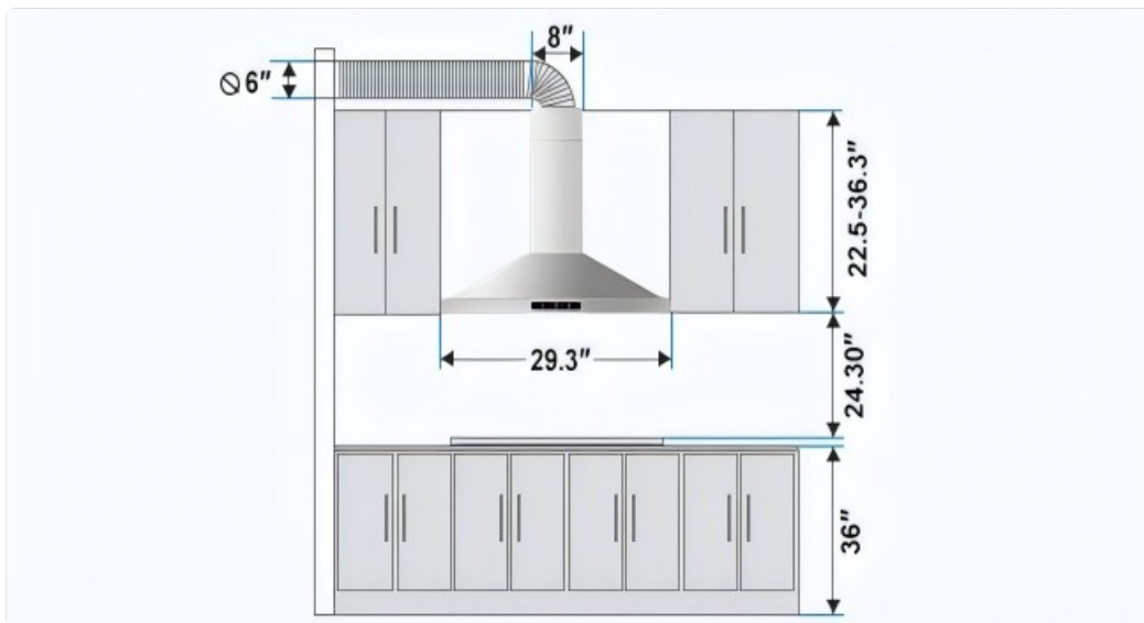
Figure 8: Ductless Installation Diagram
