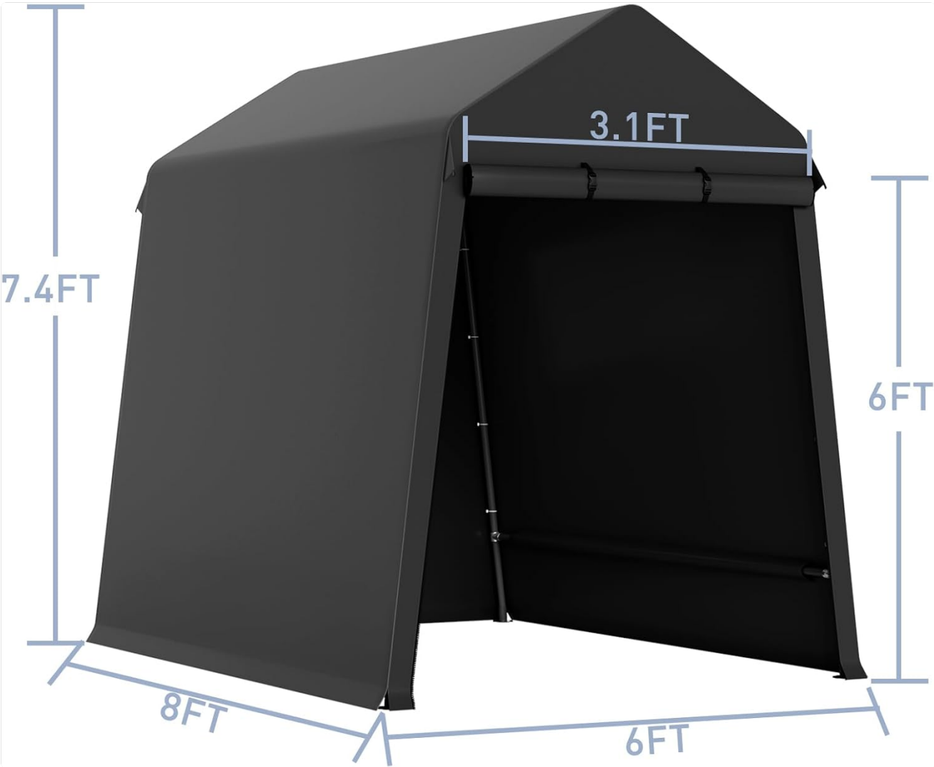
Figure 8.1: Product Dimensions. Visual representation of the shed's length, width, and height measurements.
