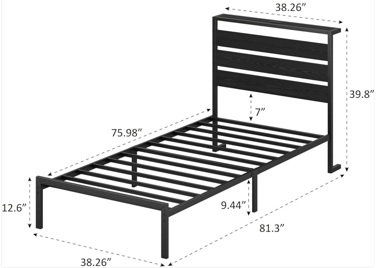
Figure 1: Dimensions of the CollaredEagle Twin Bed Frame. The frame measures approximately 81.3 inches in length, 38.26 inches in width, and 39.8 inches in height at the headboard. The under-bed clearance is 9.44 inches.
