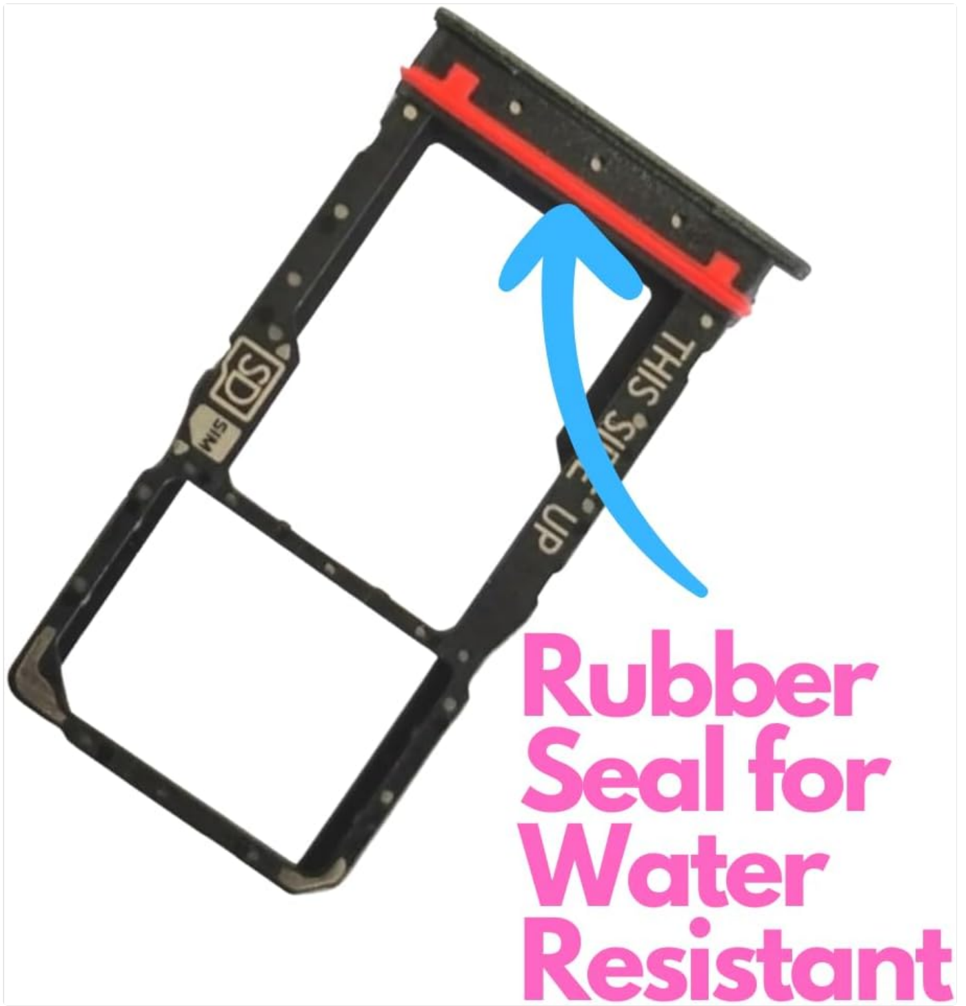
Image: Detail of the SIM card tray highlighting the integrated rubber seal, which contributes to the phone's water resistance.
