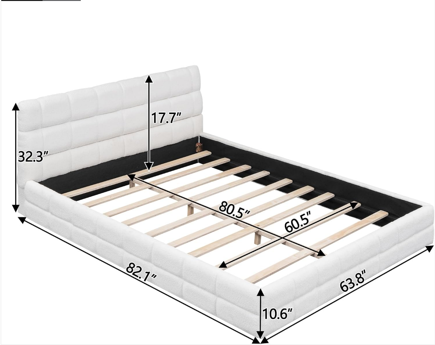
Image: Detailed dimensions of the Queen Size Upholstered Platform Bed Frame.
