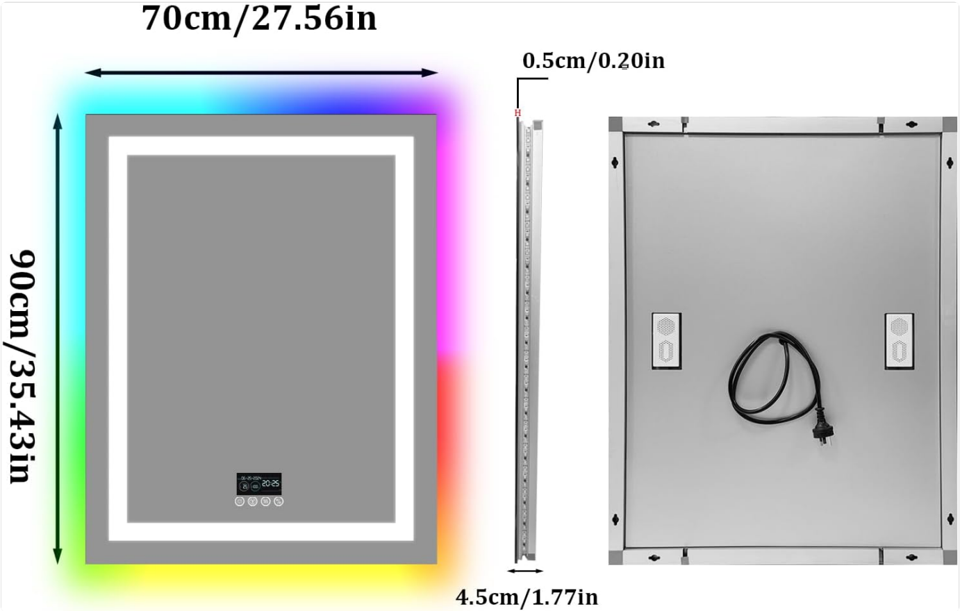
Image 4.1: Detailed dimensions of the mirror unit.
