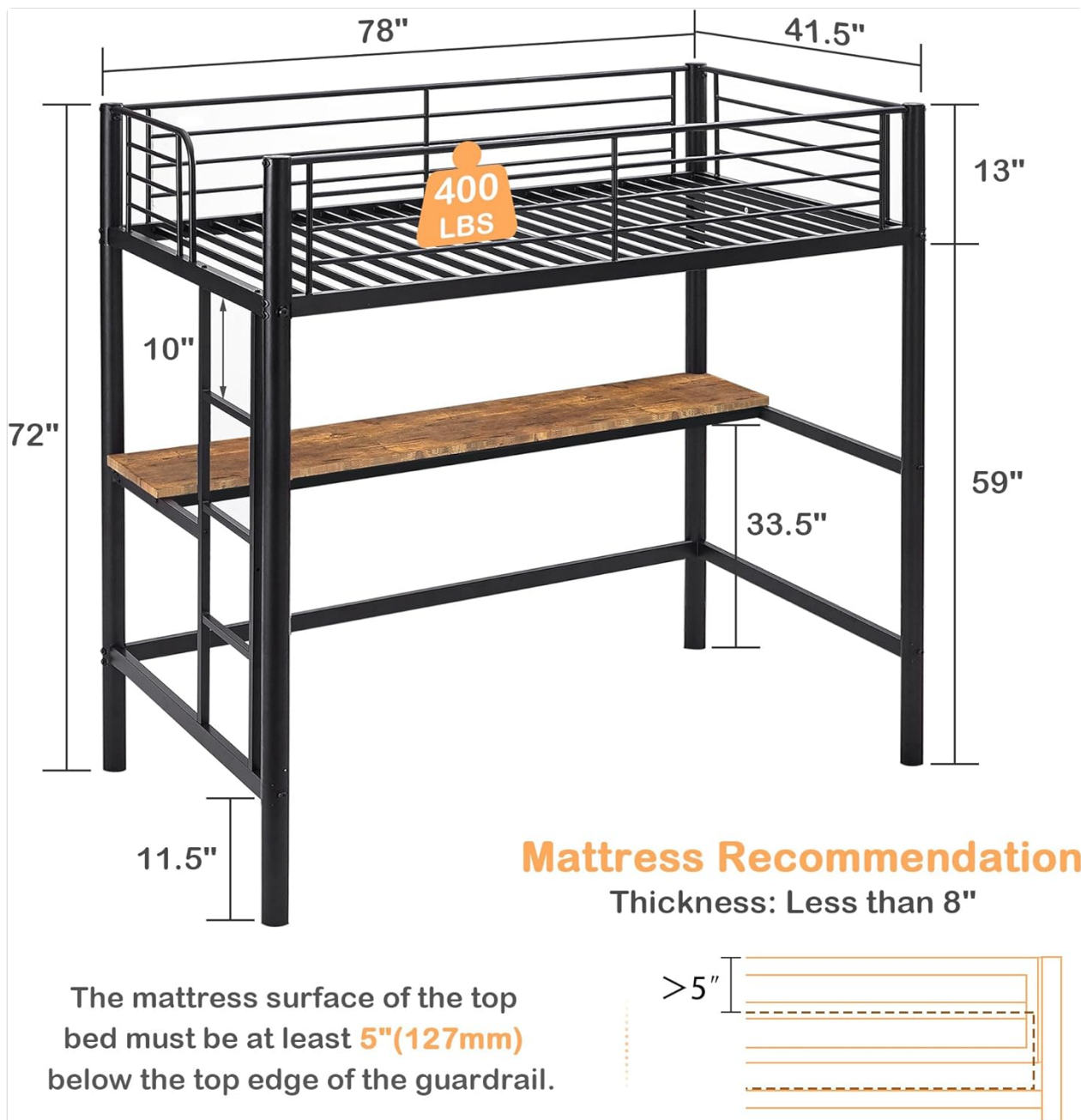
Image: Detailed dimensions of the VECELO Loft Bed.
