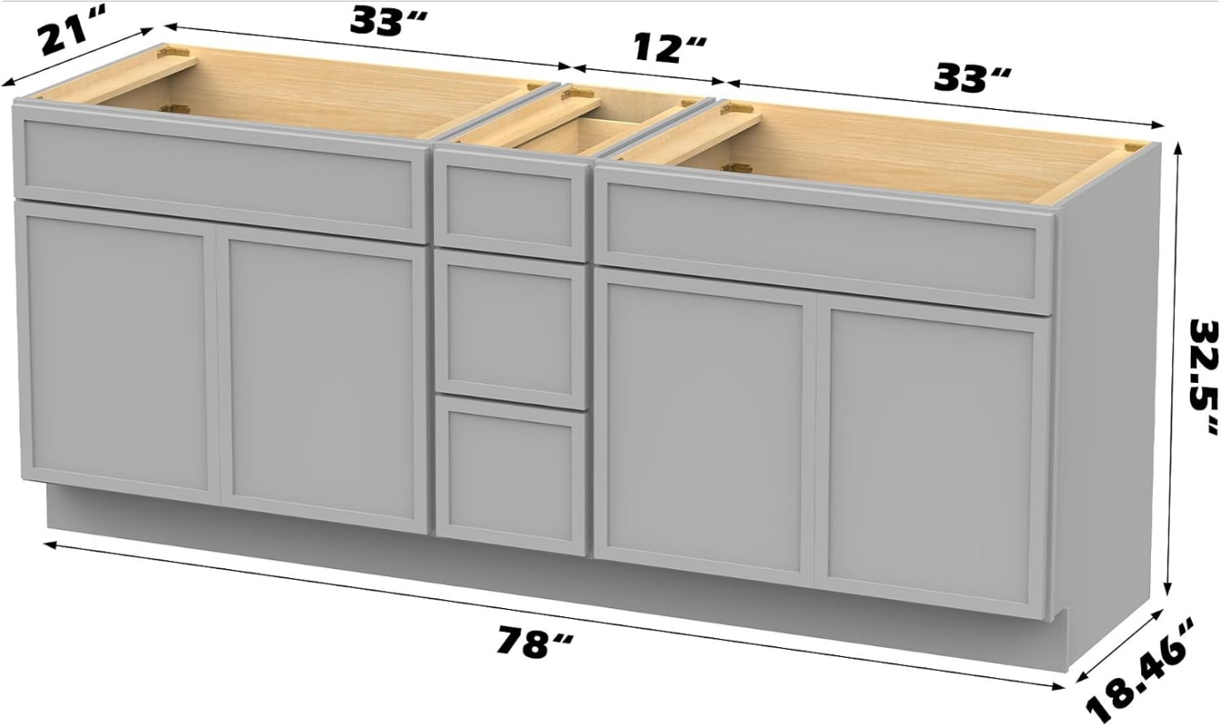
Image 7.1: Detailed dimensions of the 78-inch vanity base cabinet.
