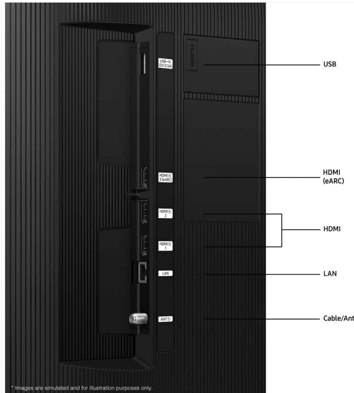
Detailed view of the rear input panel of the Samsung QLED TV, indicating USB, HDMI (including eARC), LAN, and Cable/Antenna ports.
