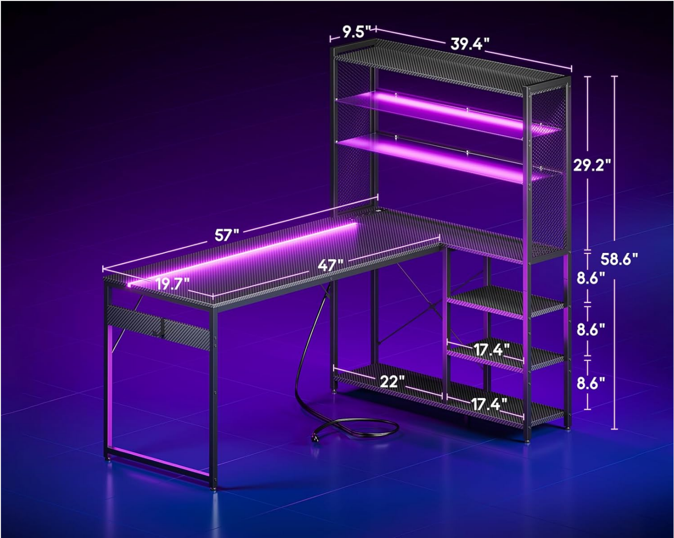
Image: Technical diagram illustrating the overall dimensions of the L-shaped desk, including the length and width of the main desktop, the height of the monitor stand, and the dimensions of the integrated shelving units.
