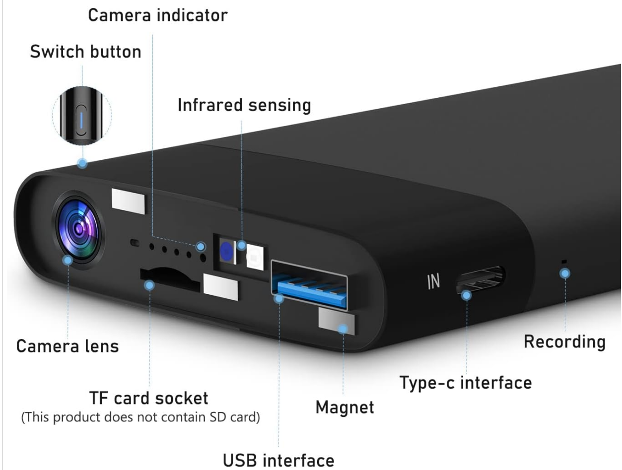
Figure 3.2: Detailed Component View
