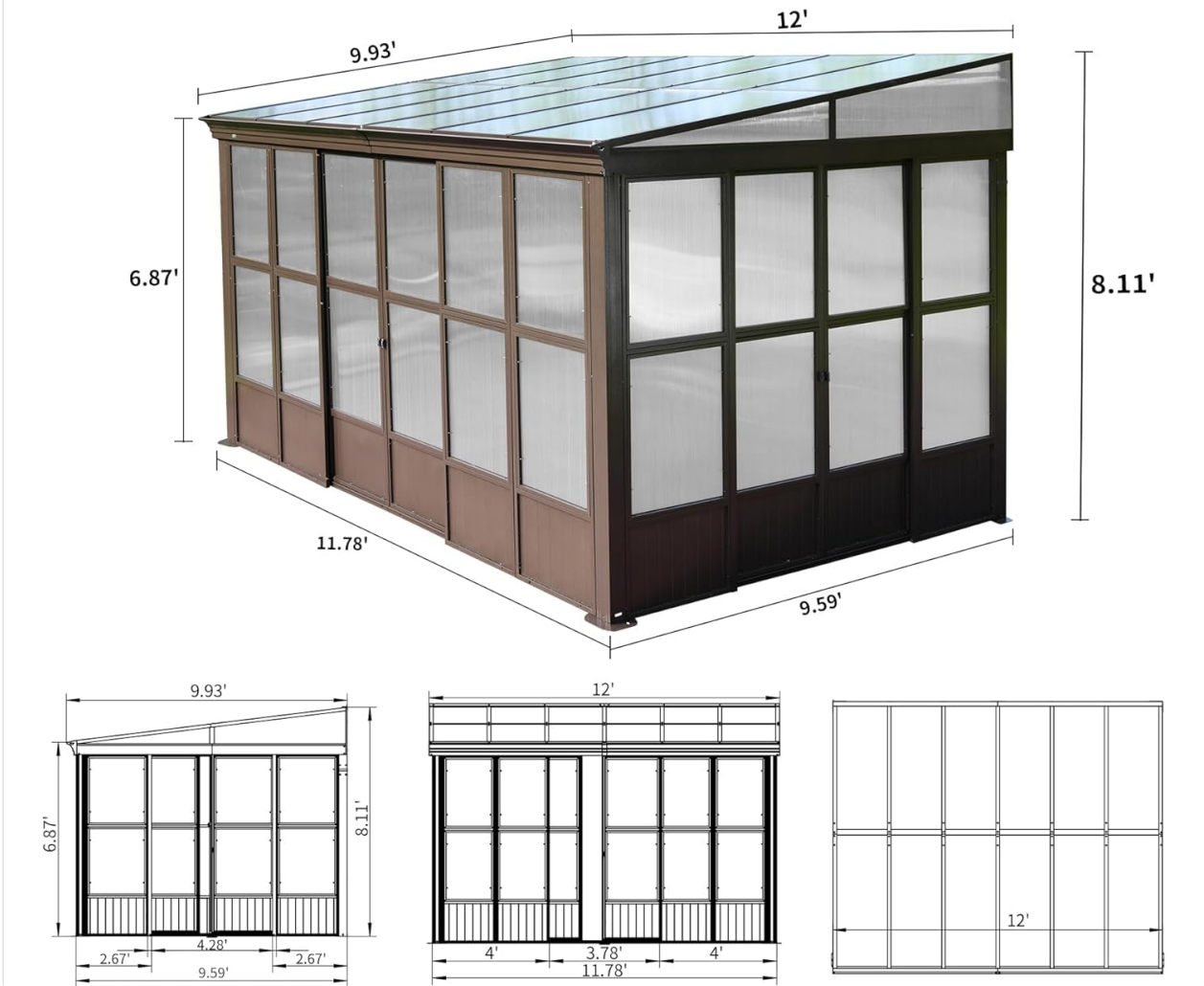
Image 6.1: Dimensional drawing of the Domi Lean-to Sunroom, showing length, width, and height measurements.
