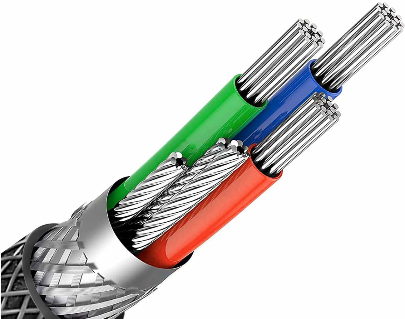
Figure 7.1: Illustration of the high-quality copper wire and internal construction, ensuring stable and fast performance.
