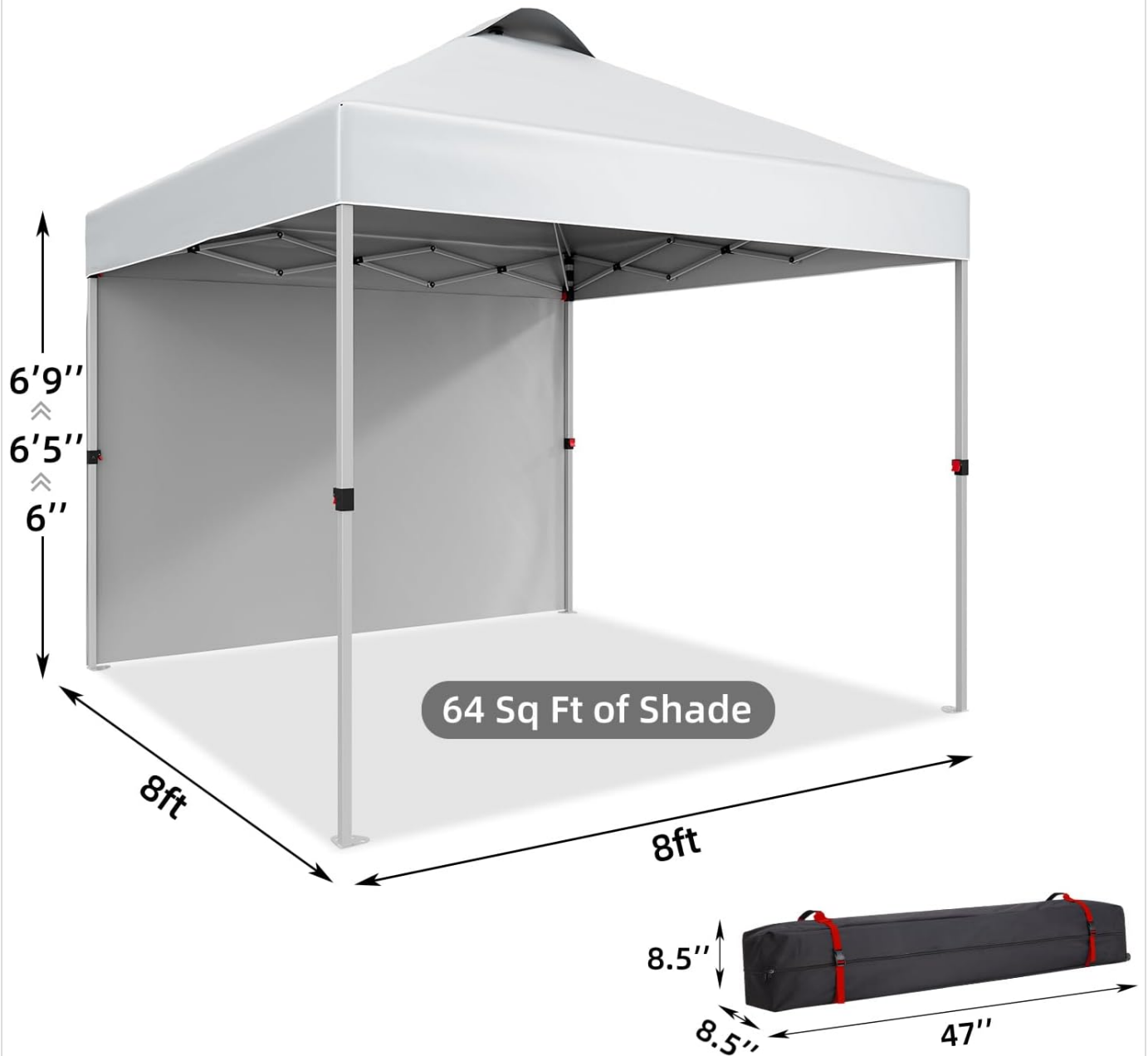
Figure 7.1: Canopy Dimensions
