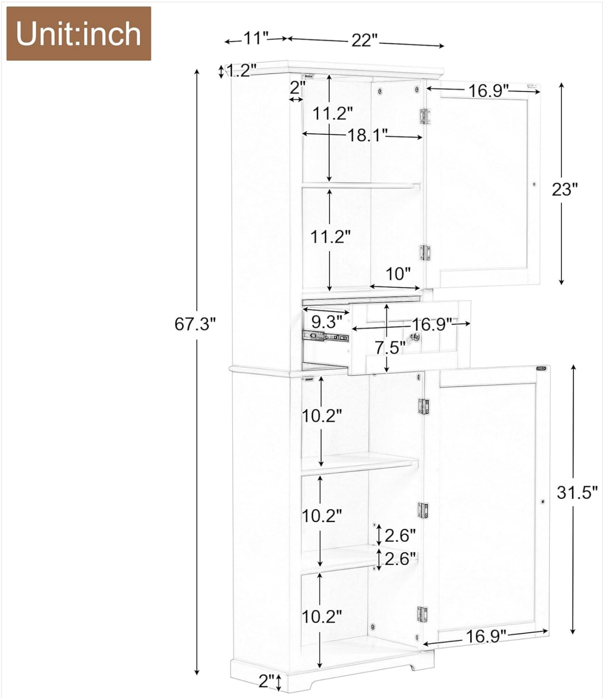
Image: Technical diagram illustrating the precise dimensions of the cabinet, including overall height (67.3 inches), width (22 inches), depth (11 inches), and internal measurements for shelves and drawer.
