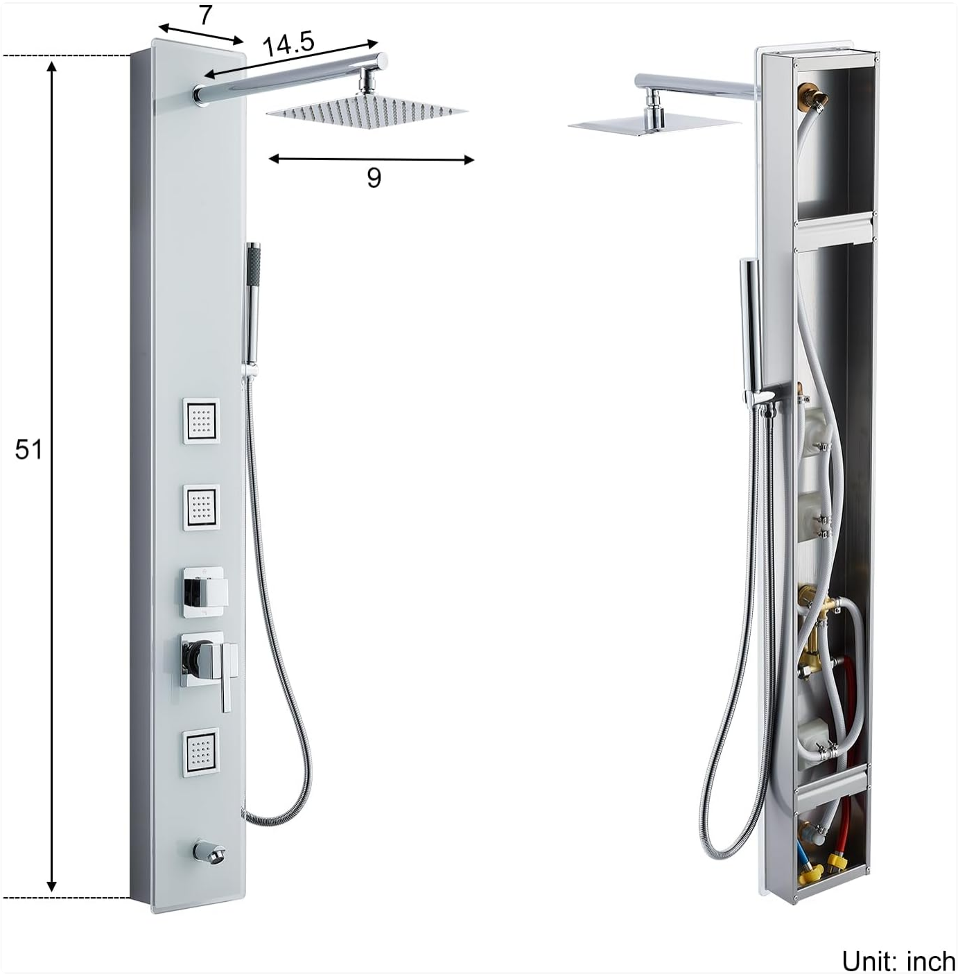
Figure 3: Product dimensions in inches for the MENATT Shower Panel Tower System.
