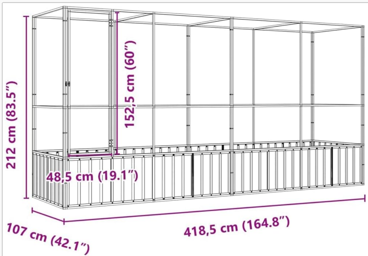
Figure 1: Aviary Dimensions Diagram. This diagram illustrates the overall width, depth, and height of the aviary, along with the dimensions of the main access door.
