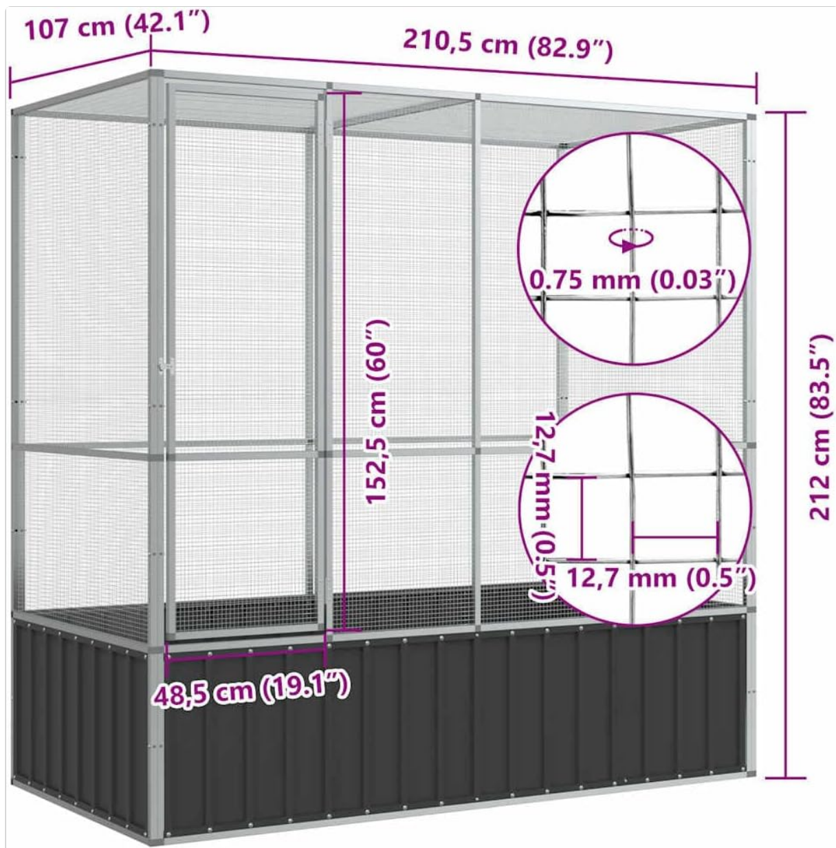
Figure 3: Detailed dimensions of the aviary, including overall size, door size, and grid/mesh dimensions.
