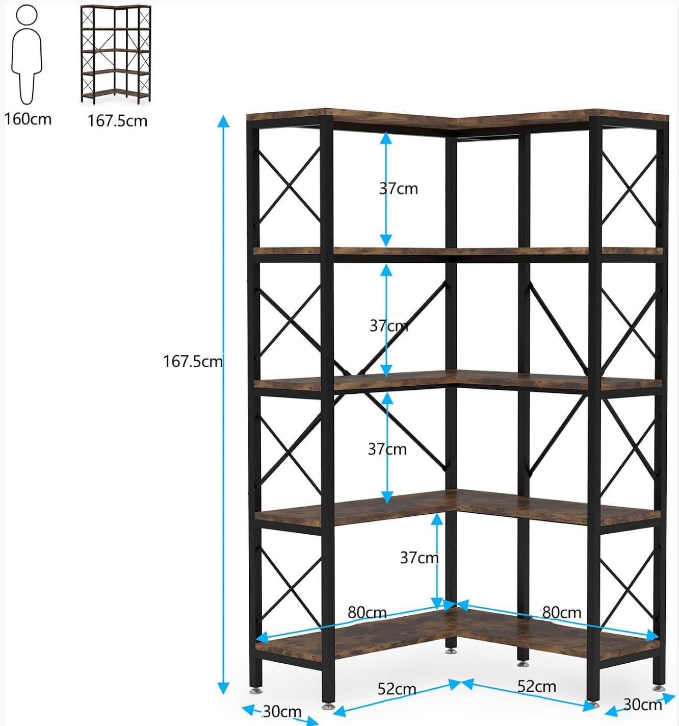
Image: A diagram illustrating the overall dimensions and internal shelf spacing of the corner bookshelf.
