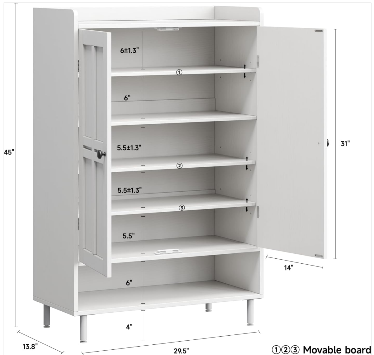
Image: Detailed dimensions and adjustable shelf options for the cabinet.
