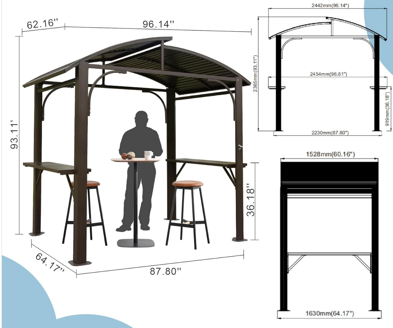
Figure 2: A technical diagram illustrating the overall dimensions of the 8'x5' Arc Roof Grill Gazebo, including height, length, and width, along with detailed measurements for various structural elements.
