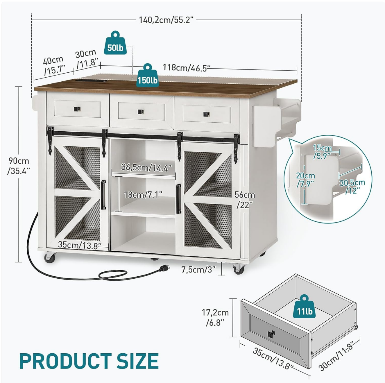
Figure 2: Detailed product dimensions, including overall size and internal measurements for drawers and shelves.
