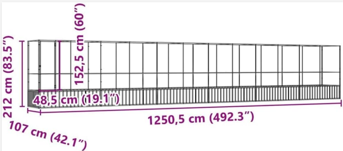
Image 4.1: Diagram illustrating the overall dimensions of the aviary, crucial for planning placement and assembly.
