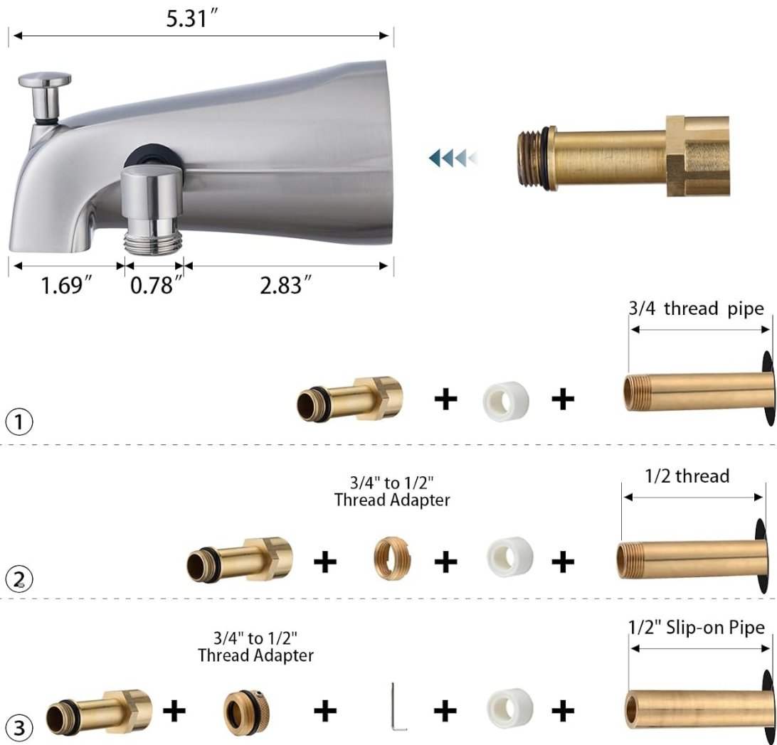
Image: Diagram illustrating the universal fit options for connecting the faucet to different pipe sizes.
