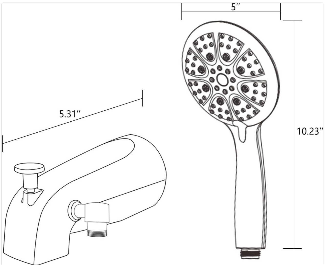
Image: Detailed dimensions of the tub spout and handheld showerhead for reference.
