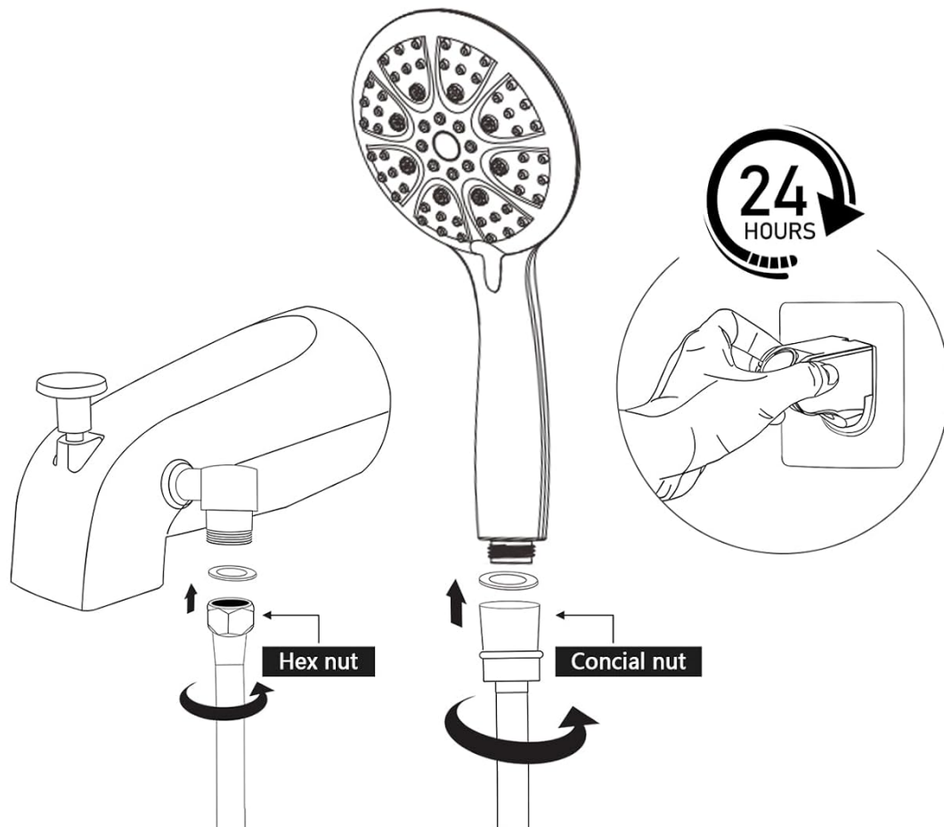
Image: Visual guide for connecting the handheld shower hose to the tub spout and securing the shower holder.
