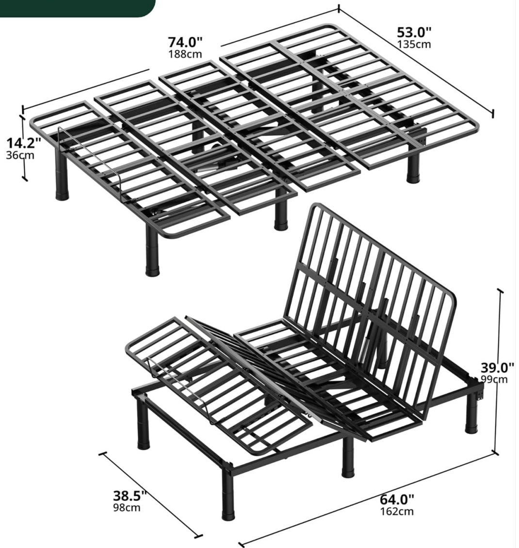
Image: Detailed dimensional drawing for the Full size bed frame.
