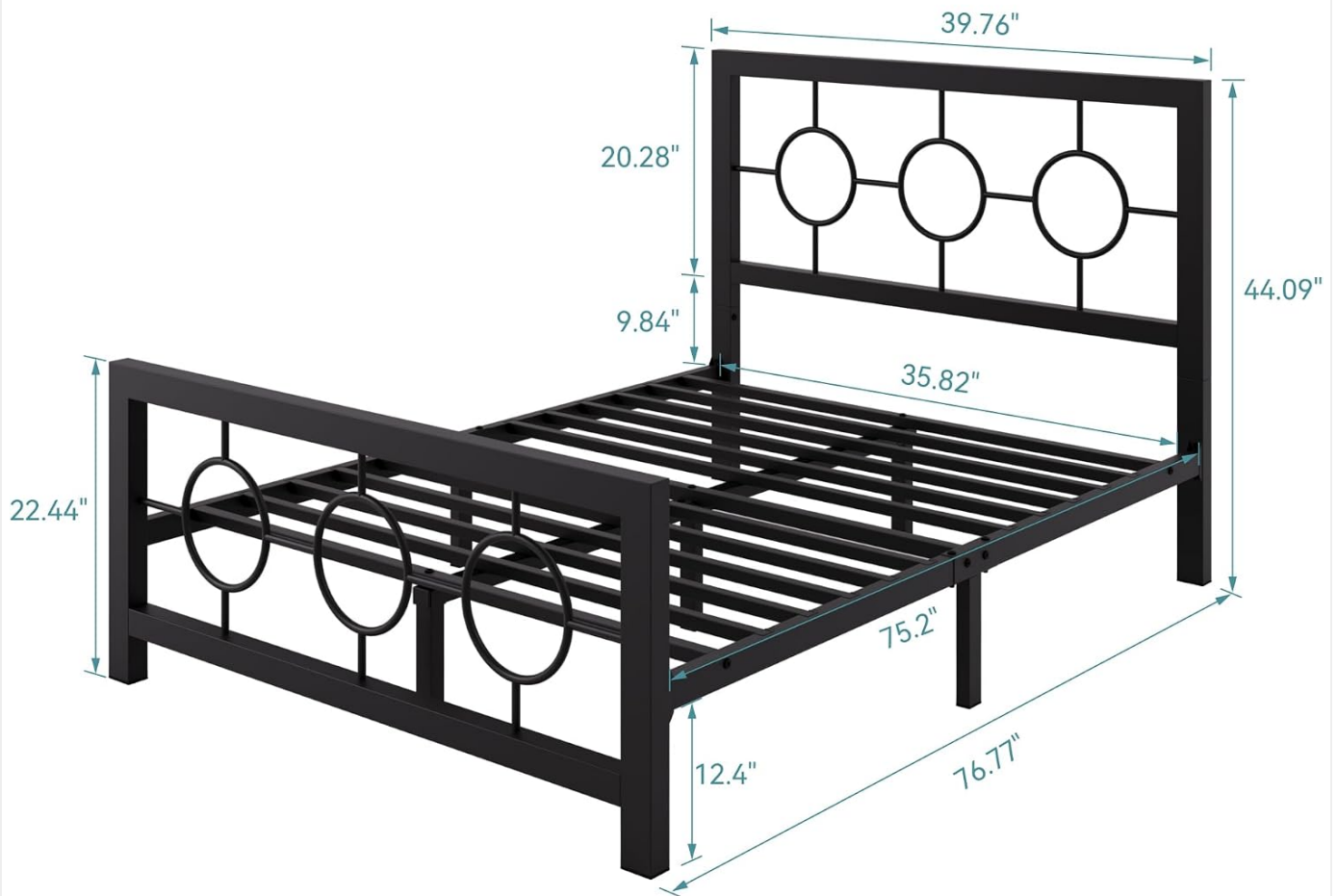
Image: Dimensional diagram of the Twin Size bed frame, showing overall length, width, and height.
