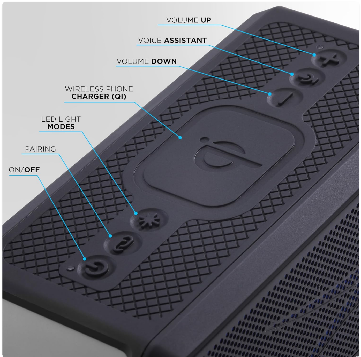
Detailed view of the HydraBLAST 2.0 control panel, illustrating the various buttons for power, volume, and feature control.
