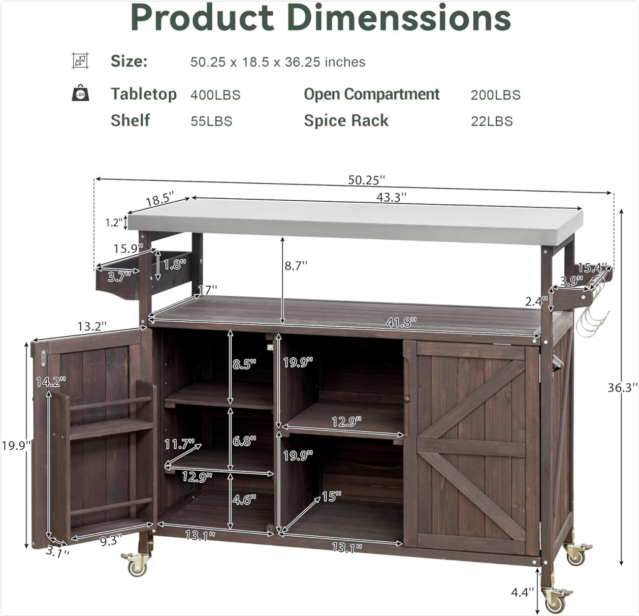
Figure 2: Product dimensions and weight capacities for various sections of the grill table.
