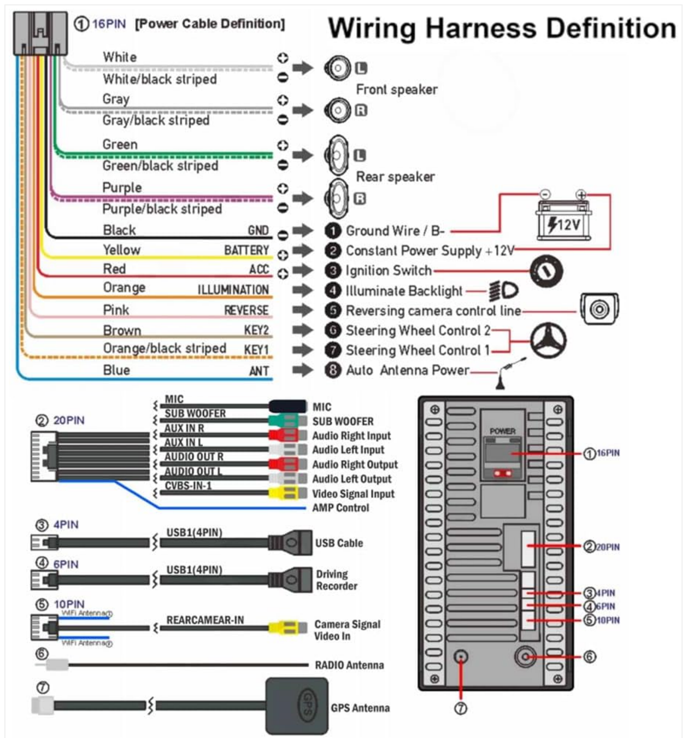
Figure 5: Detailed wiring harness definition for the car stereo, showing connections for power, speakers, and other functions.
