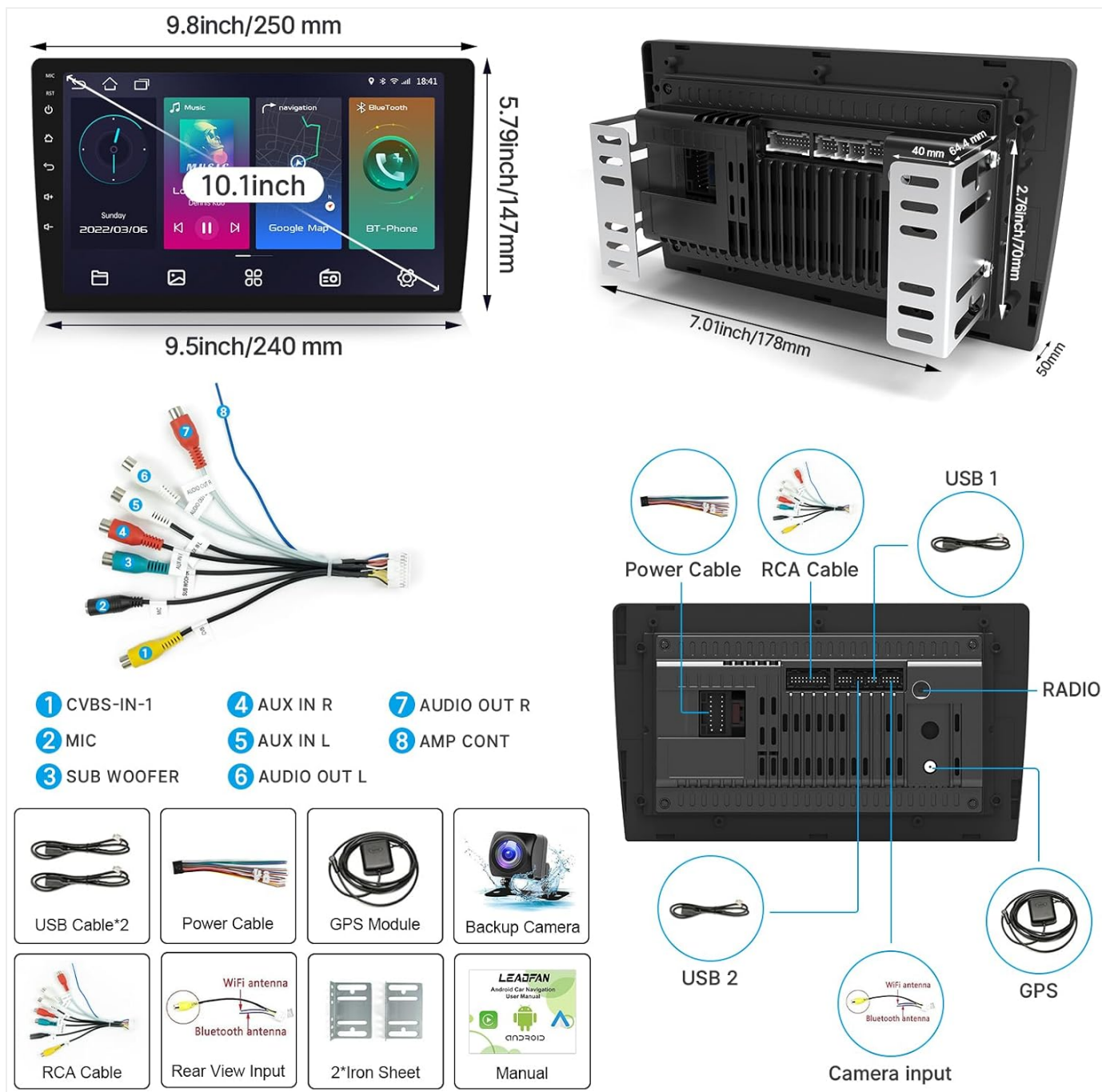
Figure 3: Product dimensions and included accessories for installation.
