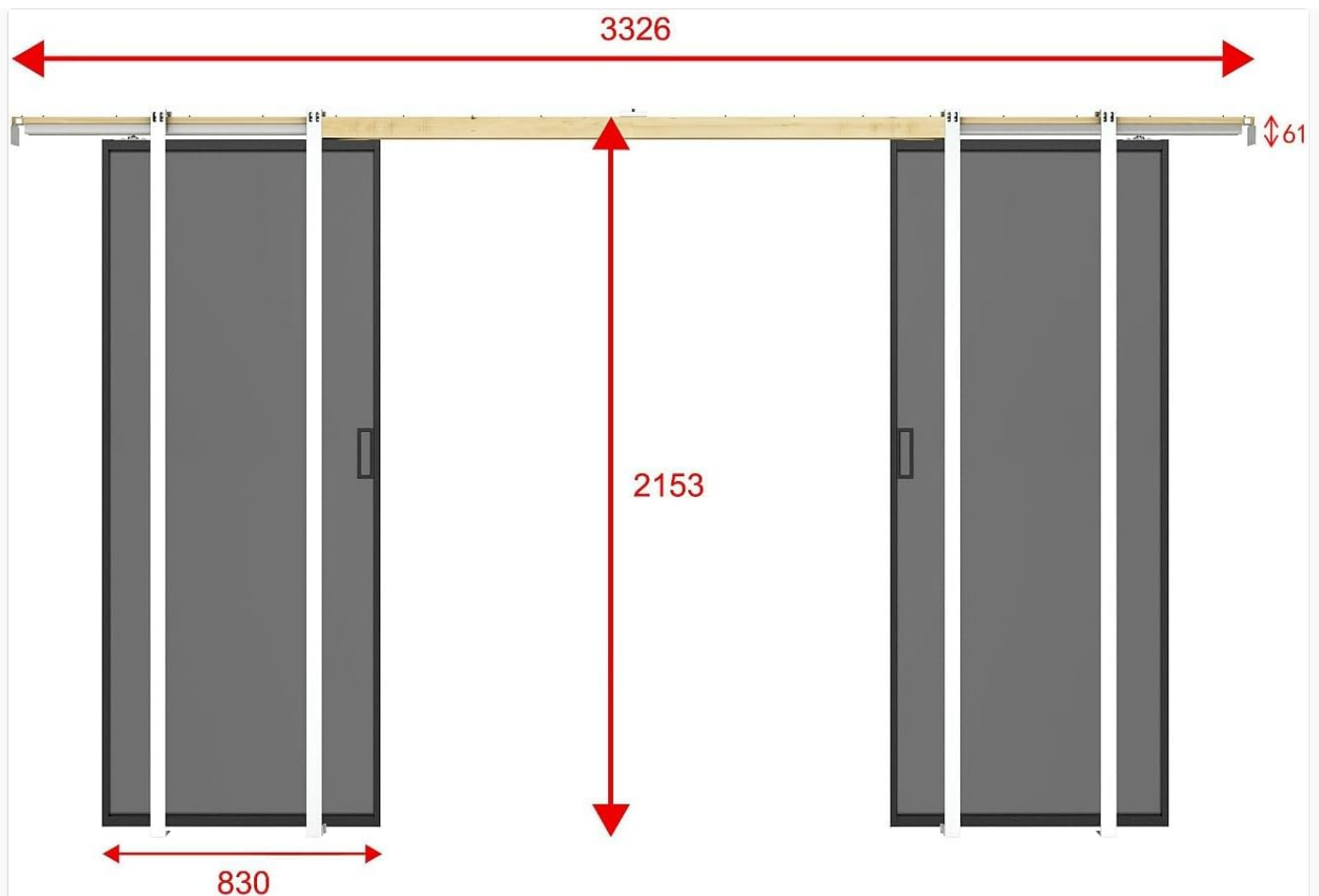
Image 2: Dimensional diagram of the LINCI II double sliding pocket door system.
