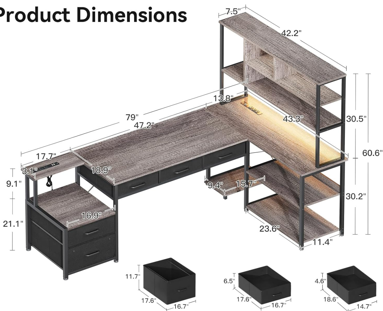
Figure 2: Product Dimensions for Assembly Reference.
