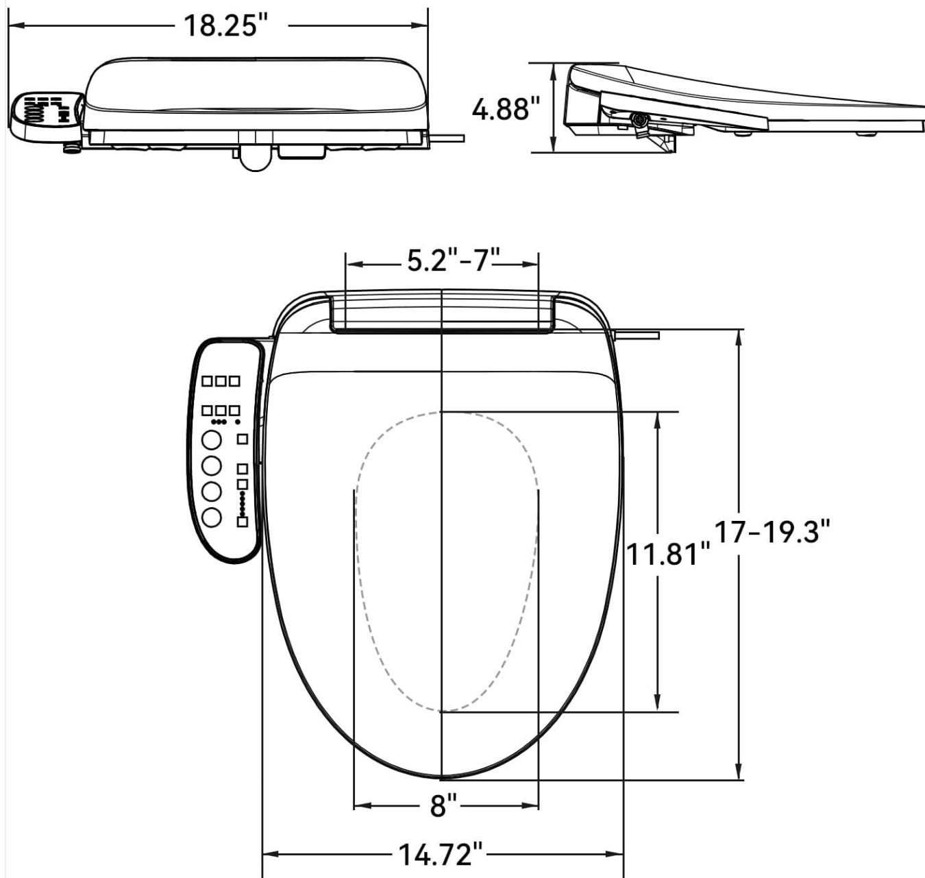
Image 9.1: Detailed technical drawing showing the dimensions of the HOROW B0403 bidet toilet seat, including length, width, and height measurements.
