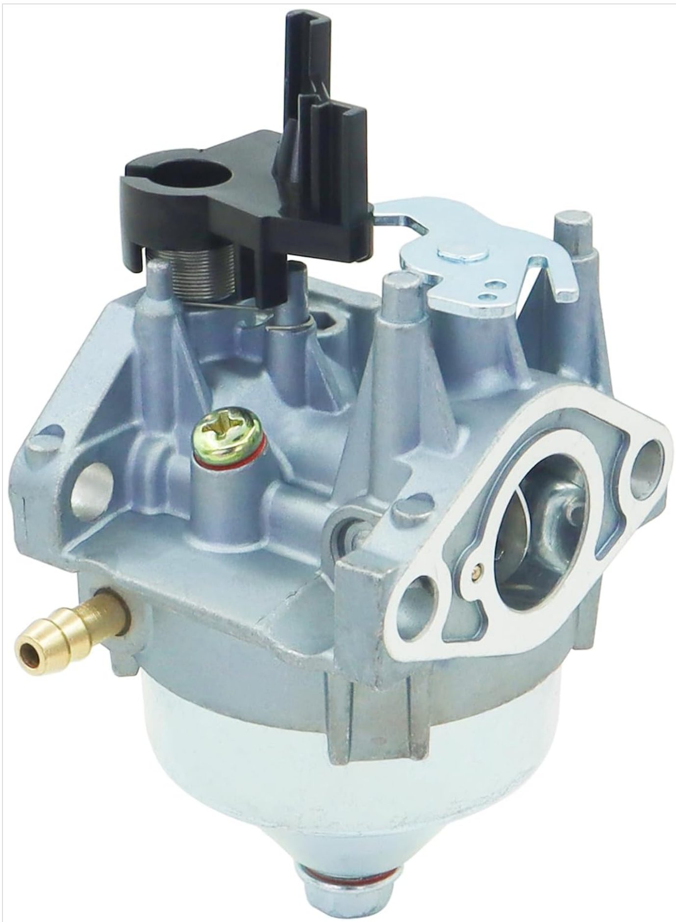
Figure 1: Front view of the DABAZUALY 11A-B2AQ723 TB 160 Carburetor, showing the fuel inlet and choke mechanism.
