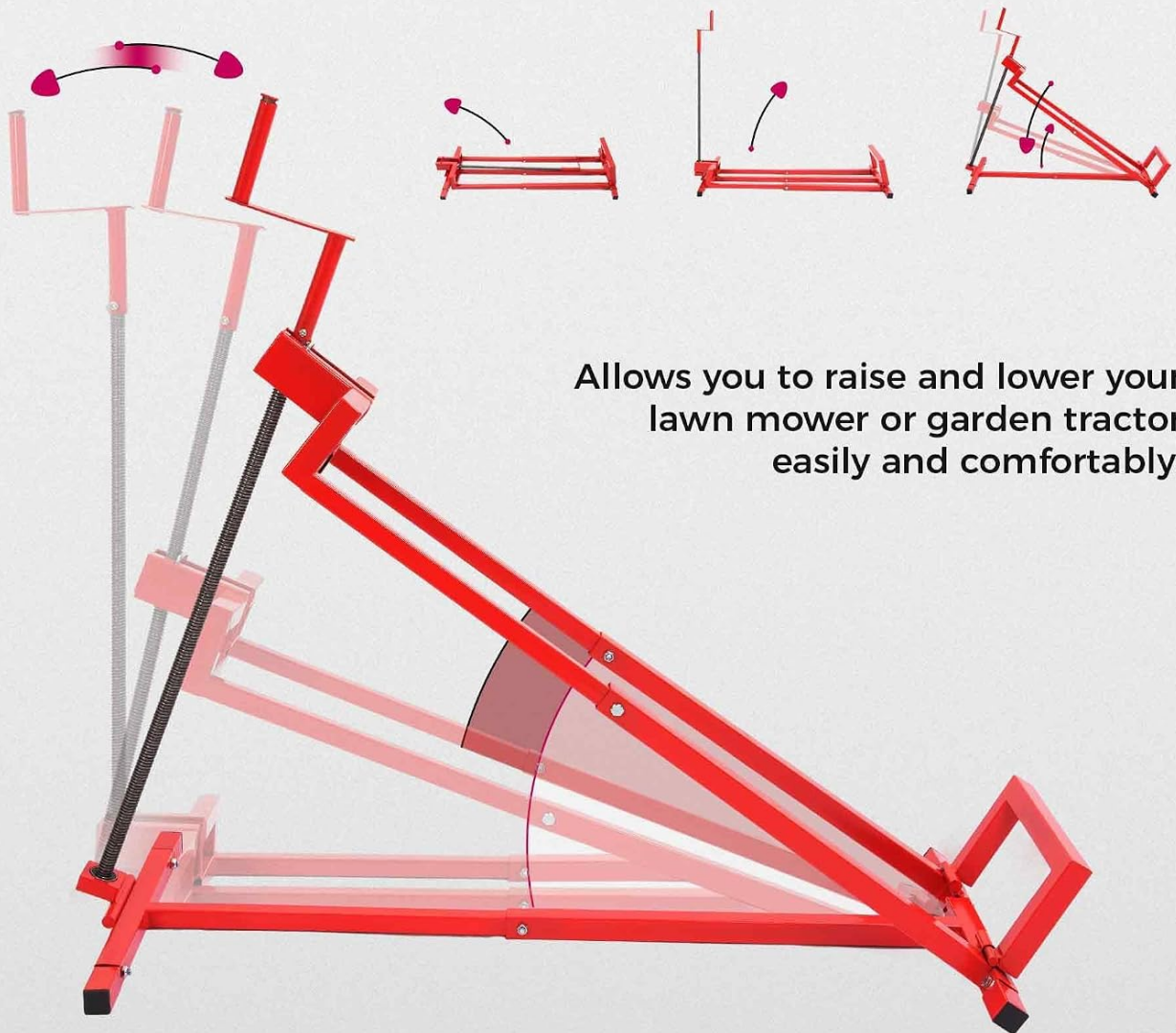
Figure 6: The lift jack allows for controlled raising and lowering of your equipment.
